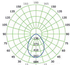
Curva fotometrica Distribution curve 10W
