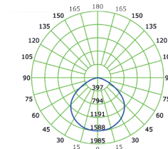
Curva fotometrica Distribution curve 50W
