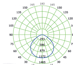
Curva fotometrica Distribution curve 30W
